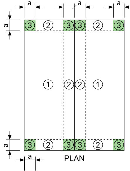
Figure 2.0 Gable Roof Zone Designations
